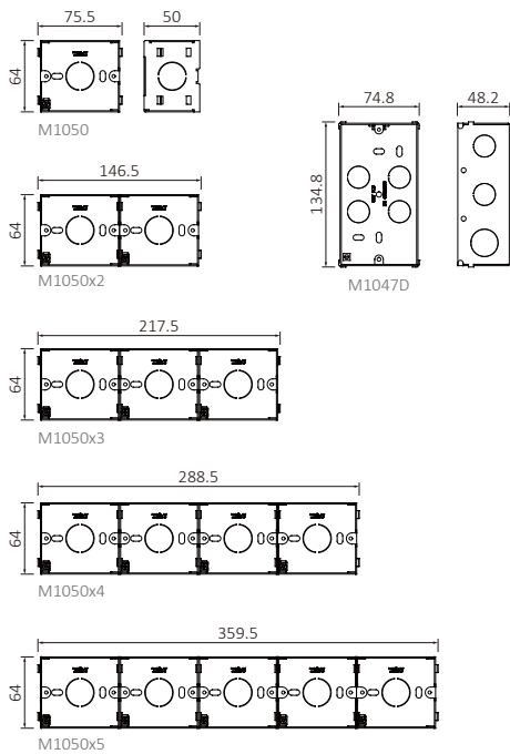
Metal (Flush Mounting)
