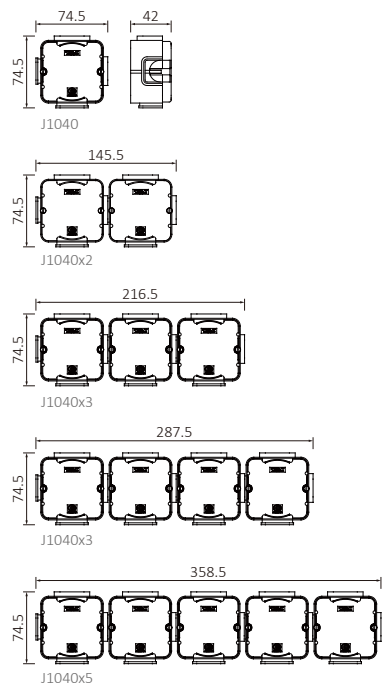
Plastic (Flush Mounting)
